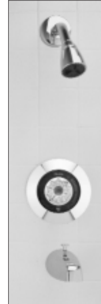
Bath and shower pressure balance mixing valve, integral checkstops, temperature limit stop, reversible inlets, acrylic handle, slip-on spout, and 2.5 gpm (9.5 L/m) showerhead. (P909HJ1S shown)
